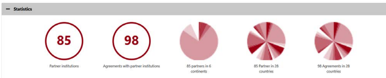
Figure 7 - Statistics
