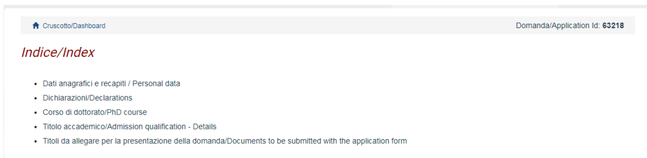
Fig. 5 – Application Sections
